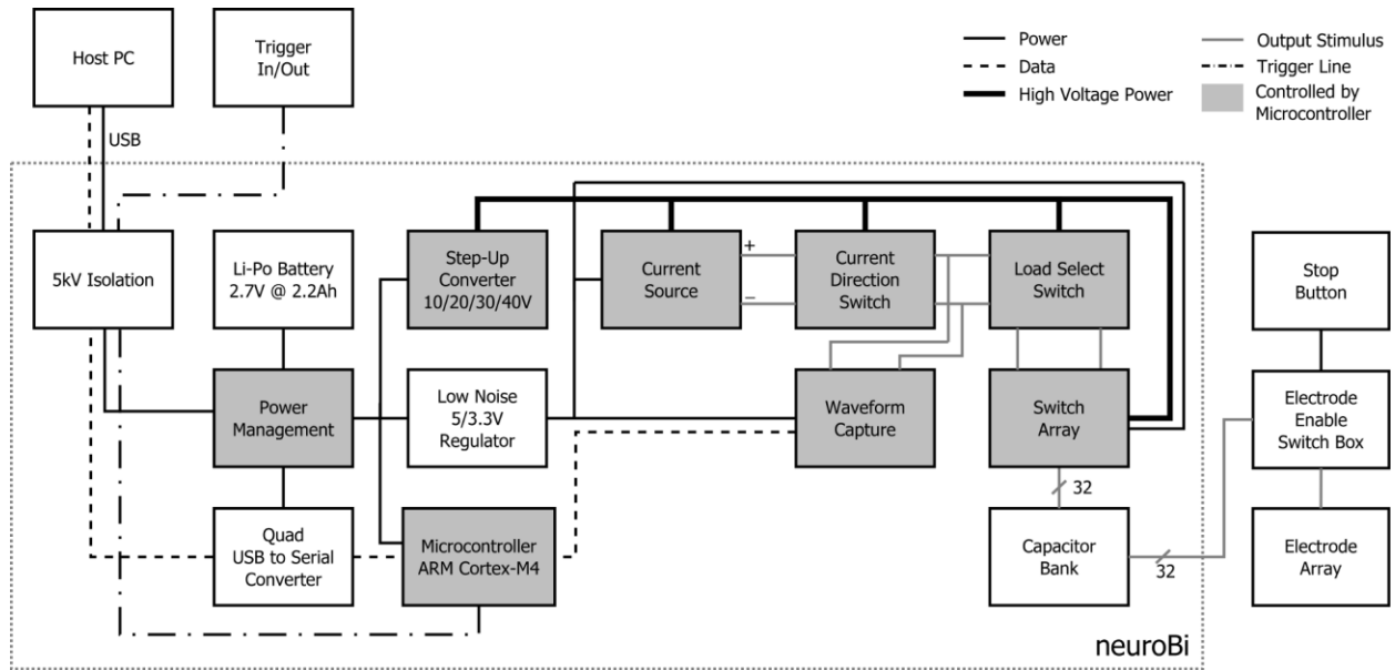
FIGURE 3. Block diagram illustrating the major functional components of neuroBi and its place within a typical patient-testing setup.
