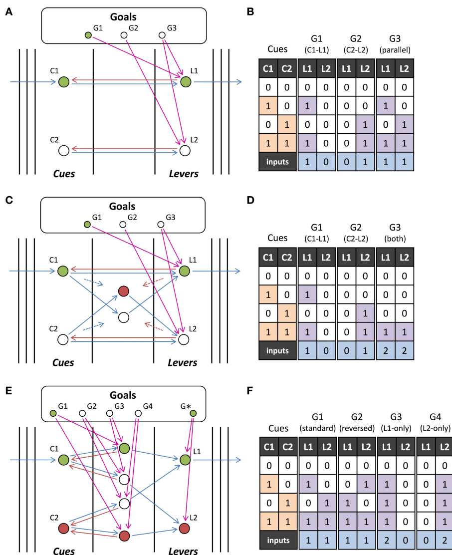
FIGURE 6 | Stimulus-response Tasks. (A) An example of how the cortical architecture would be utilized for a stimulus-response task where a subject pulls one of two levers when presented with one of two sensory cues. The task switches between one of three “goals”: lever L1 should be pulled for cue C1 and cue C2 ignored (G1), L2 for C2 and C1 ignored (G2), and L1 for C1 and L2 for C2 (G3). Network activity is shown for when G1 is active. Similarly, the arrows to the cue units from the left and those leaving the lever units depict the inputs and outputs of the network (i.e., only “active” connections) for a particular set of inputs. (B) Input-output tables for the network shown in (A) for the three different goals. The final row indicates the number of inputs
