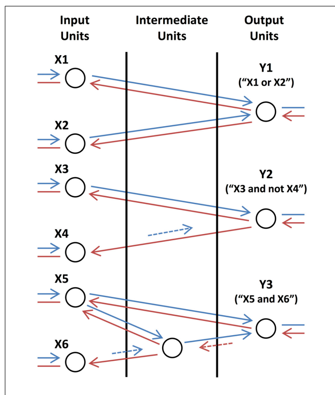
FIGURE 3 | Basic Logic Motifs. From top to bottom, motifs in which the output units compute the operations “X1 or X2,” “X3 and not X4,” and “X5 and X6,” respectively. Arrows correspond to feedforward (blue) and feedback (red) connections with short (dashed and shorter length) and long (solid and longer length) time lags. Arrows are also shown connecting the input units to lower-level units (not shown) and connecting the output units to higher-level units (not shown) as these motifs function as circuits in a larger network.
