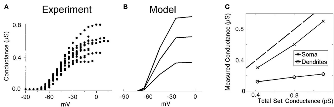
FIGURE 3 | Low-threshold potassium conductance as a function of membrane voltage. (A) Experimental results showing voltage-clamp experiments for a number of real octopus cells. The conductance is calculated for a range of voltage-clamp levels. The maximum conductance is taken as the highest level of conductance (at the most depolarized voltages). (B) Model results with the low-threshold potassium channels located in both the dendrites and the soma as previously described. The three lines are associated with three different low-threshold potassium
