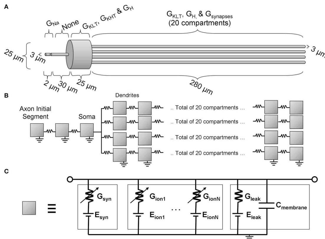
FIGURE 2 | The octopus cell model. (A) The morphology with an indication of the locations of active ion channels. (B) The model topology showing the locations of each compartment (illustrated as a gray box). (C) The equivalent circuit representation of each compartment.
