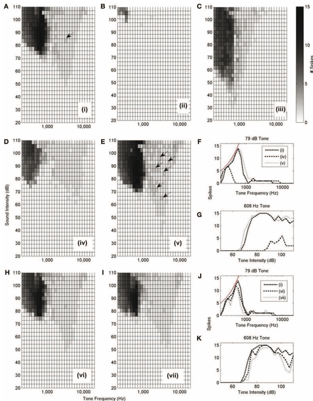
FIGURE 12 | (A–E, H, and I): Model responses to tones of different frequencies and intensities. In all cases, 300 ANFs were used as input. The innervation profile is indicated by the roman numeral designation, as depicted in Figure 10 . The arrows highlight the presence of double action potentials in relevant sub-figures. The shaded bar shows the number of spikes recorded in response to the 25 ms tone with 2.5 ms ramp onset and offset. A response of 12 spikes corresponds to 480 Hz. However, a
